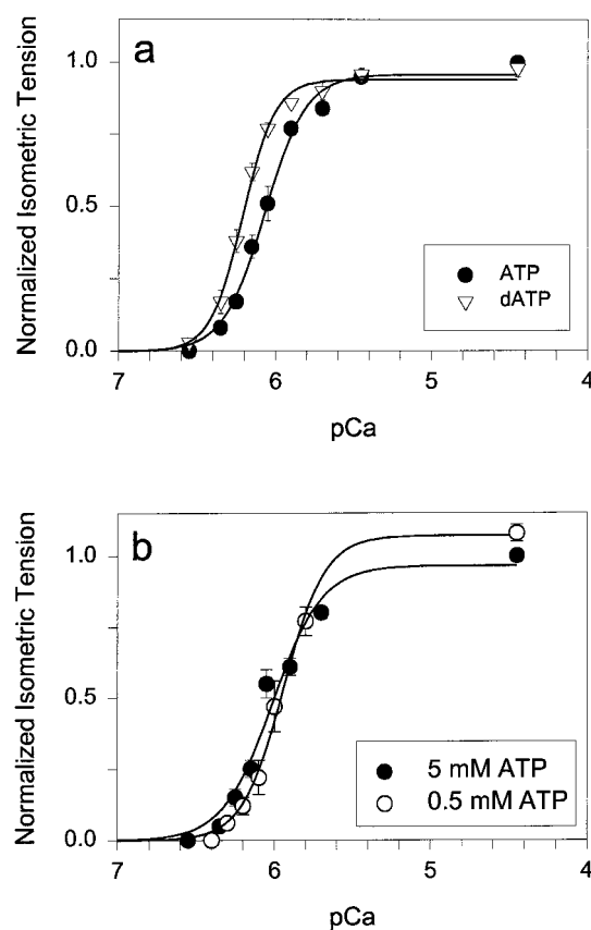
FIGURE 2 Relationship between pCa and steady-state tension. Values are normalized means \pm SE for comparison of 5 mM ATP (●) with 5 mM dATP (▽; 10 fibers) or 0.5 mM ATP (○, 9 fibers), and the data were fit with the Hill equation (solid lines). In a the fit values for half-maximum tension (pK) and slope ( n ) were 6.06 \pm 0.02 and 3.3 \pm 0.3 (mean \pm SE) for 5 mM ATP versus 6.21 \pm 0.01 and 4.2 \pm 0.3 for 5 mM dATP, with no difference in P_o . In b the fit values for 5 mM ATP were 6.00 \pm 0.04 (pK) and 2.8 \pm 0.5 ( n ) versus 5.95 \pm 0.02 (pK) and 3.3 \pm 0.3 ( n ) for 0.5 mM ATP, and P_o was increased to 1.08 \pm 0.04 ( p < 0.01 ).
